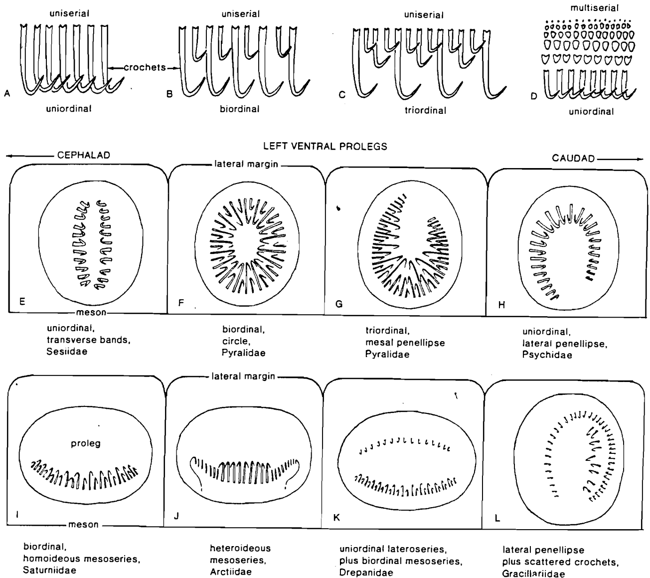
Figure 3. Crochet arrangements and terminology (Stehr, 1987).
