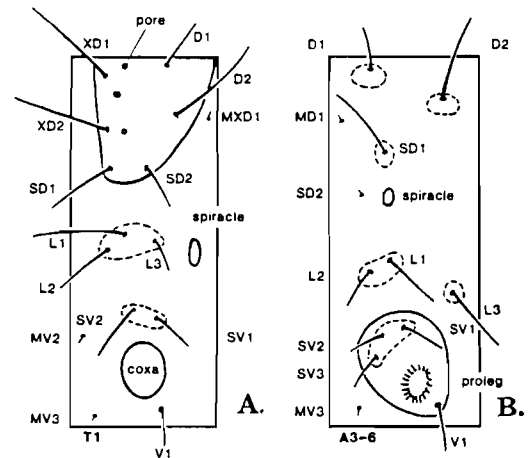
Figure 5. Typical setal maps. A. T1; B. A3-A6 (Stehr, 1987).
