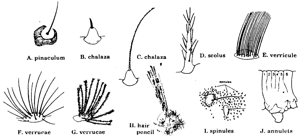
Figure 4. Cuticular and setal structures of caterpillars (A-G, I, J: Stehr, 1987; H: Peterson, 1962).
