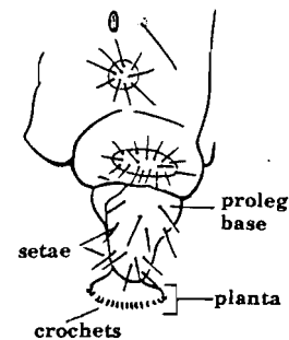
Figure 2. Abdominal proleg (Stehr, 1987).
