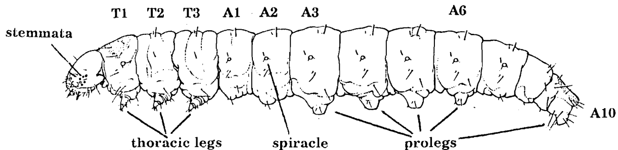
Figure 1. Basic morphological characters of Lepidopteran larvae. Pictured: Glyphipterigidae, Diploschizia habecki (from Stehr, 1987).
